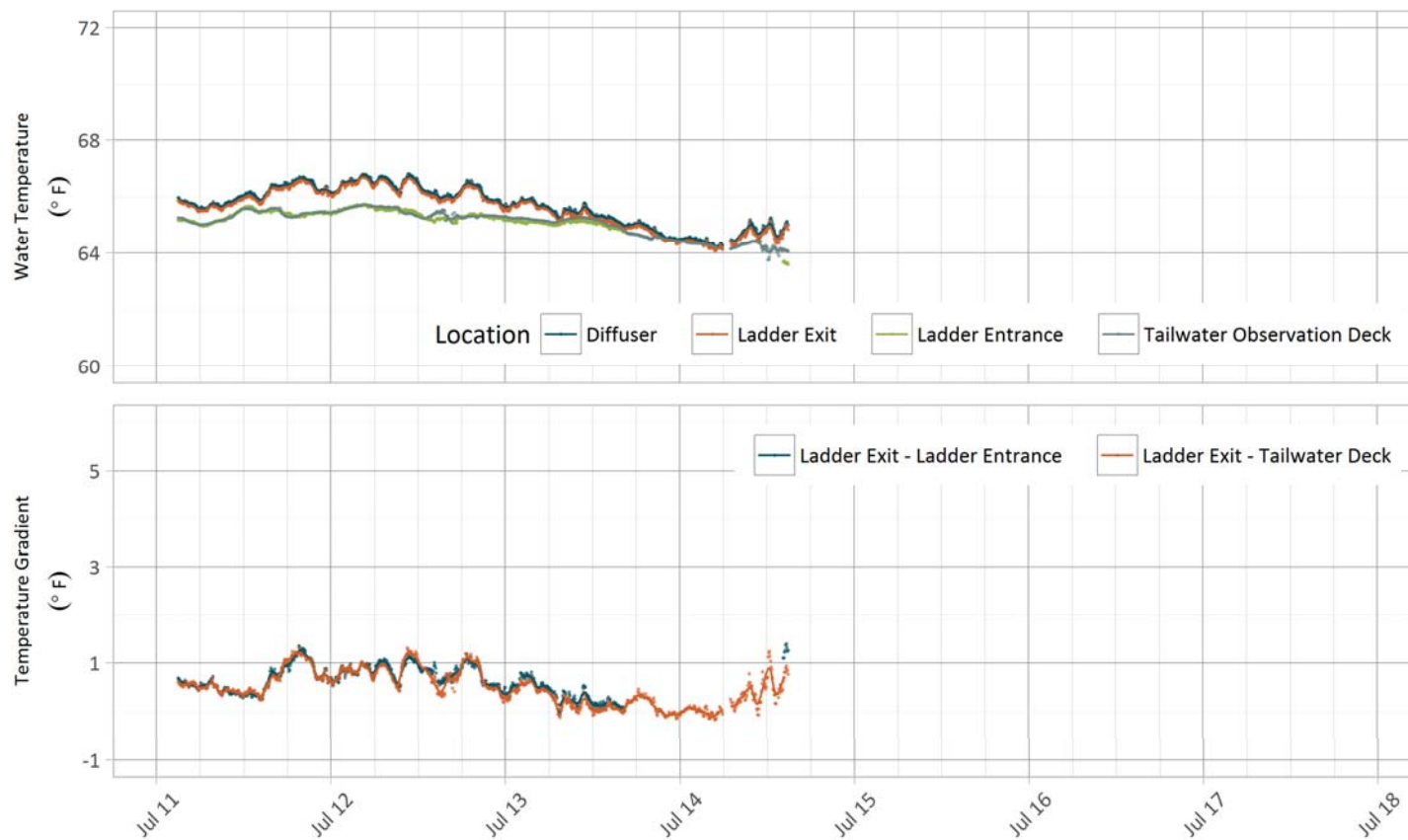
Figure 3 Water Temperatures in the Fish Ladder for Week 28
