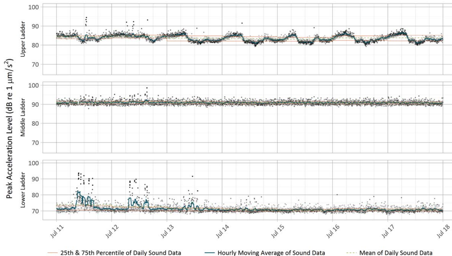
Figure 1 Peak Acceleration Levels Measured by Triaxial Accelerometers for Week 28
