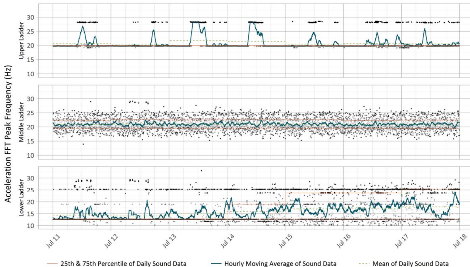
Figure 2 Acceleration Peak Frequencies Measured by Triaxial Accelerometers for Week 28
